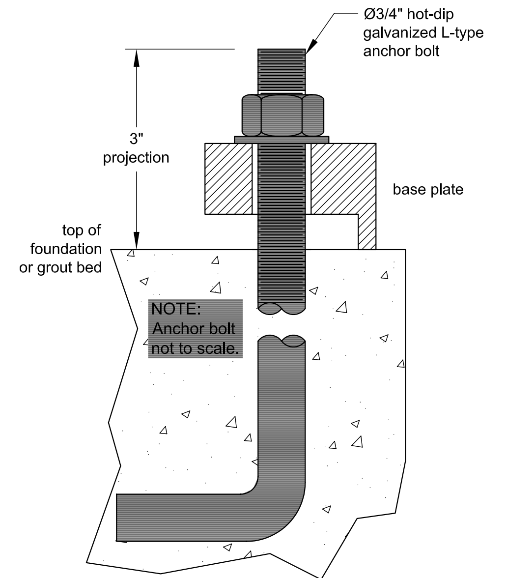
Anchorage Detail
