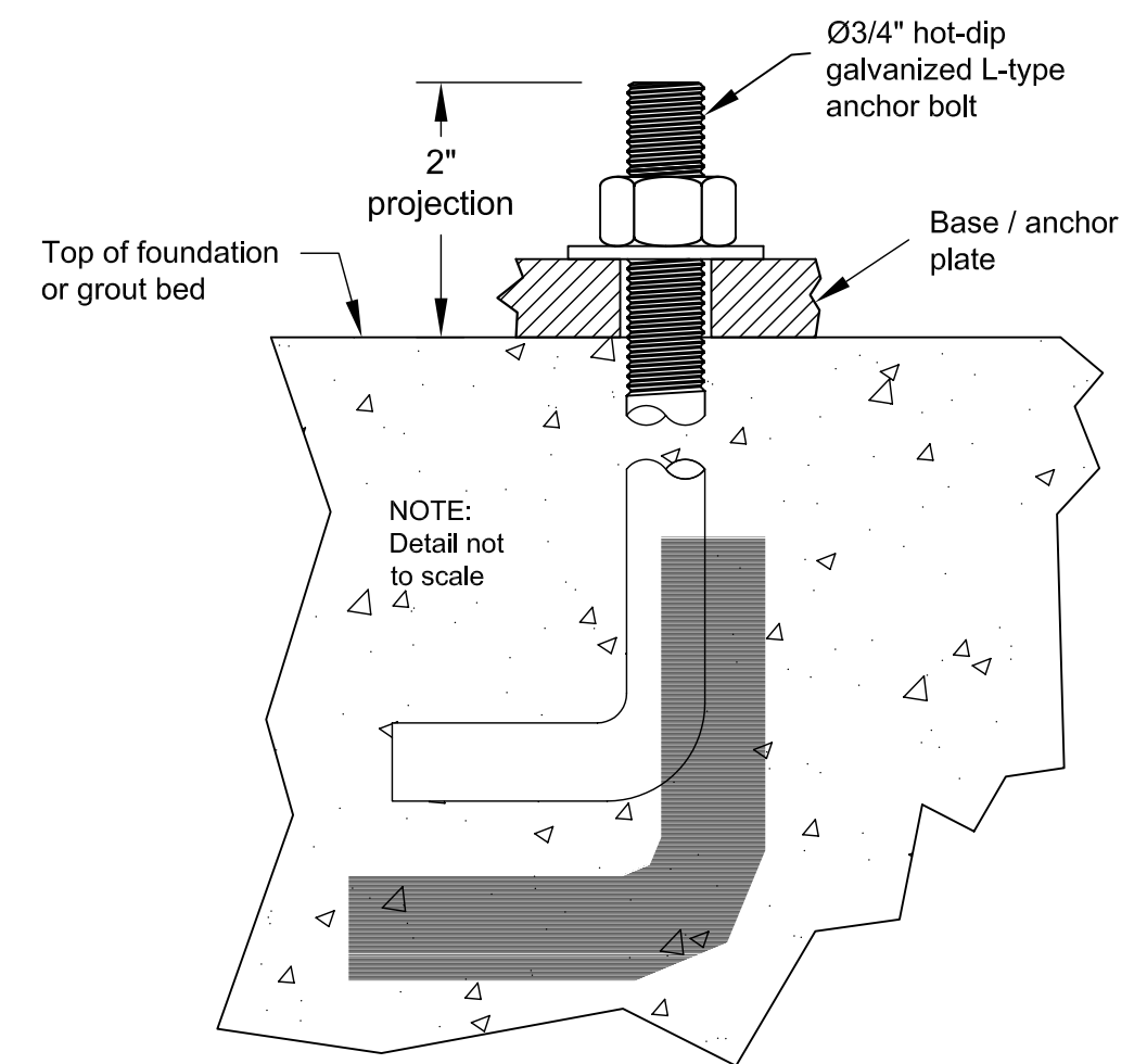
Anchorage Detail
